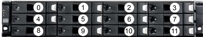
Figure 2-2 Veritas 2U12 65.5TiB/72TB Storage Shelf disk drive slot layout
